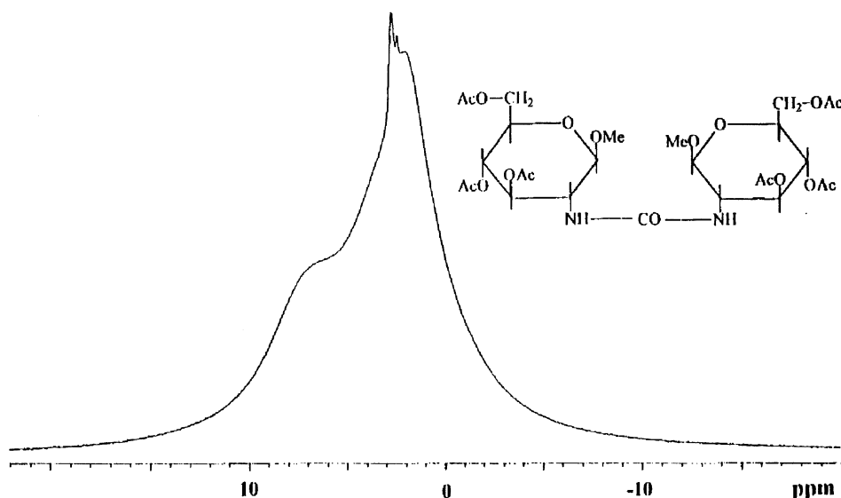
Fig. 48. ^1\text{H} MAS spectrum (at 400 MHz) of acetylated ureido sugar, rotation speed 16 kHz.
