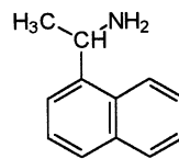
1-(1-naphthyl)-ethylamine
