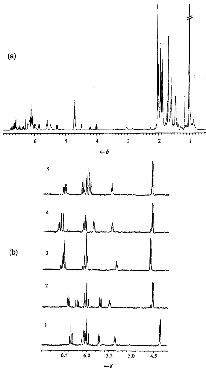
Fig. 47. (a) 400 MHz 1 H NMR spectrum of the isomeric mixture of vitamin-A-acetate and (b) continuous-flow 400 MHz 1 H NMR spectra of each isomer: 1: 11,13-di- cis -, 2: 11- cis -, 3: 13- cis -, 4: 9- cis -, 5: all- trans -vitamin A-acetate (Reprinted with permission from Ref. [114], page 1103, Copyright 1997, VCH Verlagsgesellschaft, Weinheim, and the author K. Albert).
