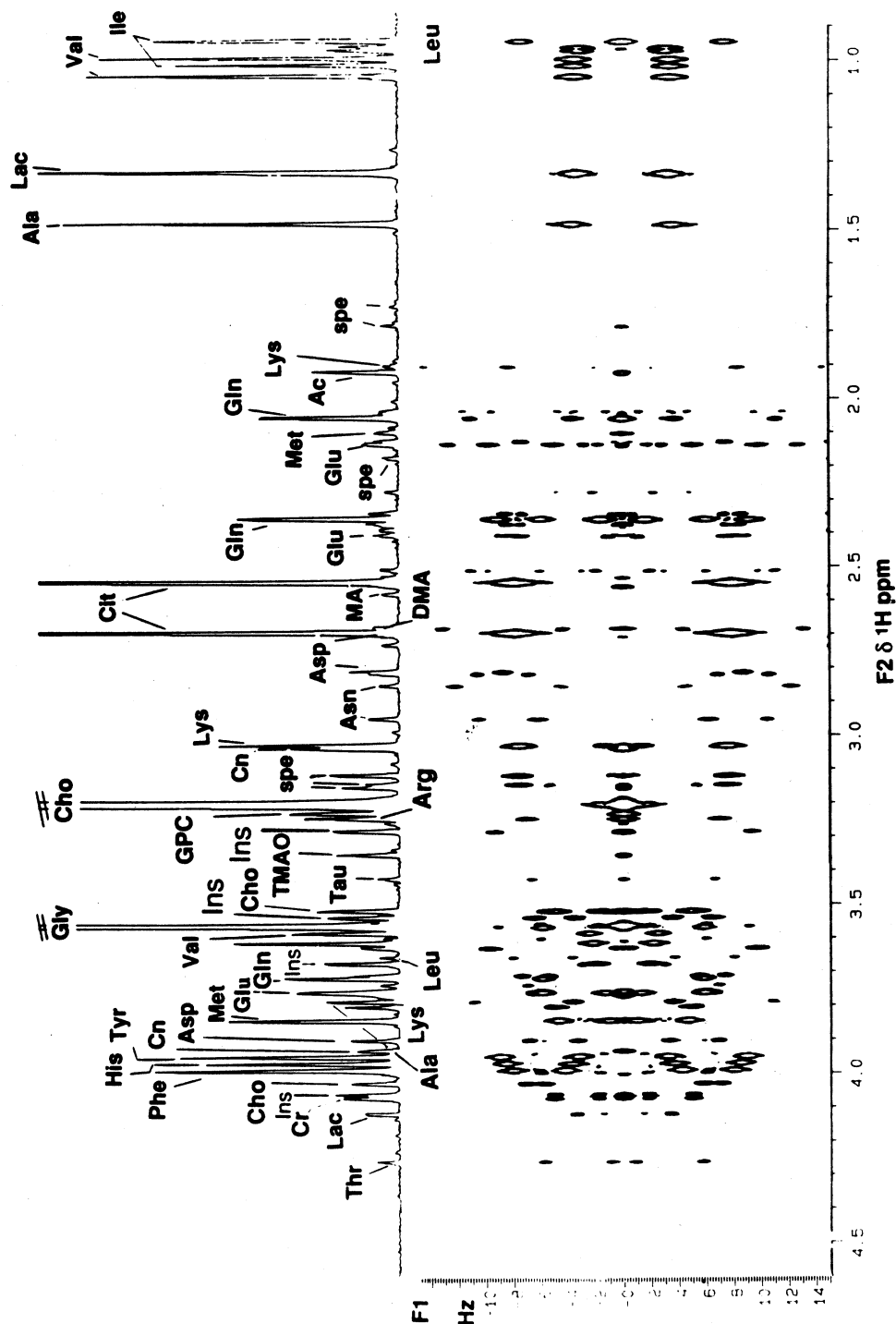
Fig. 45. 600 MHz ^1\text{H} NMR spectrum JRES of the aliphatic region of control human seminal fluid from \delta 0.9–4.6 ppm, showing contour plot and skyline F2 projection. Key: Ac, acetate; Ala, alanine; Arg, arginine; Asn, asparagine; Asp, aspartate; Cho, choline; Cit, citrate; Cr, creatine; DMA, dimethylamine; Gln, glutamine; Glu, glutamate; Gly, glycine; GPC, glycerophosphorylcholine; His, histidine; Ile, isoleucine; Ins, myo -inositol; Lac, lactate; Leu, leucine; Lys, lysine; MA, methionine; Met, methionine; Phe, phenylalanine; Spe, spermine; Tau, taurine; Thr, threonine; TMAO, trimethylamine-N-oxide; Trp, tryptophan; Tyr, tyrosine; Uri, uridine; Val, valine (Reprinted from Ref. [100], page 10, Copyright 1997) with kind permission of Elsevier Science NL, Sara Burgerhartstraat 25, 1055 KV Amsterdam, The Netherlands).
