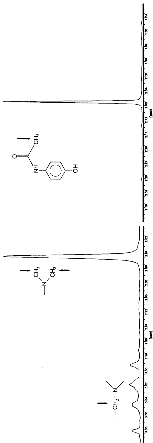
Fig. 15. ^1\text{H} NMR spectrum (expansion; 1.82–3.10 ppm) of Grippostad C, 300 MHz, solvent methanol- \text{d}_4 .
