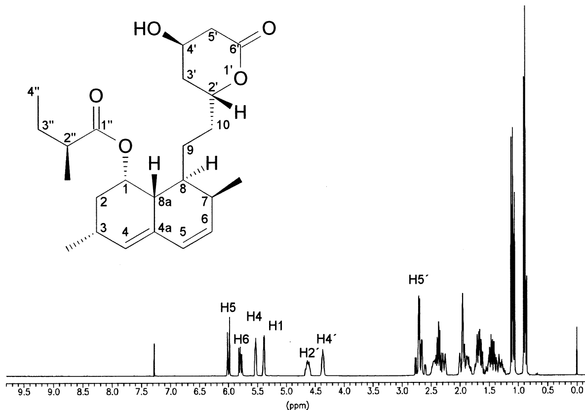
Fig. 12. ^1\text{H} NMR spectrum of lovastatin, 300 MHz, solvent \text{CDCl}_3 .
