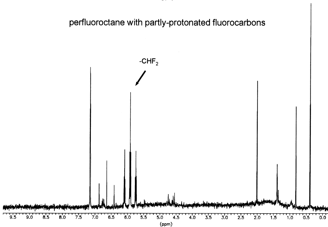
Fig. 22. Analysis of fluorocarbons, 300 MHz, neat liquid, external lock.
