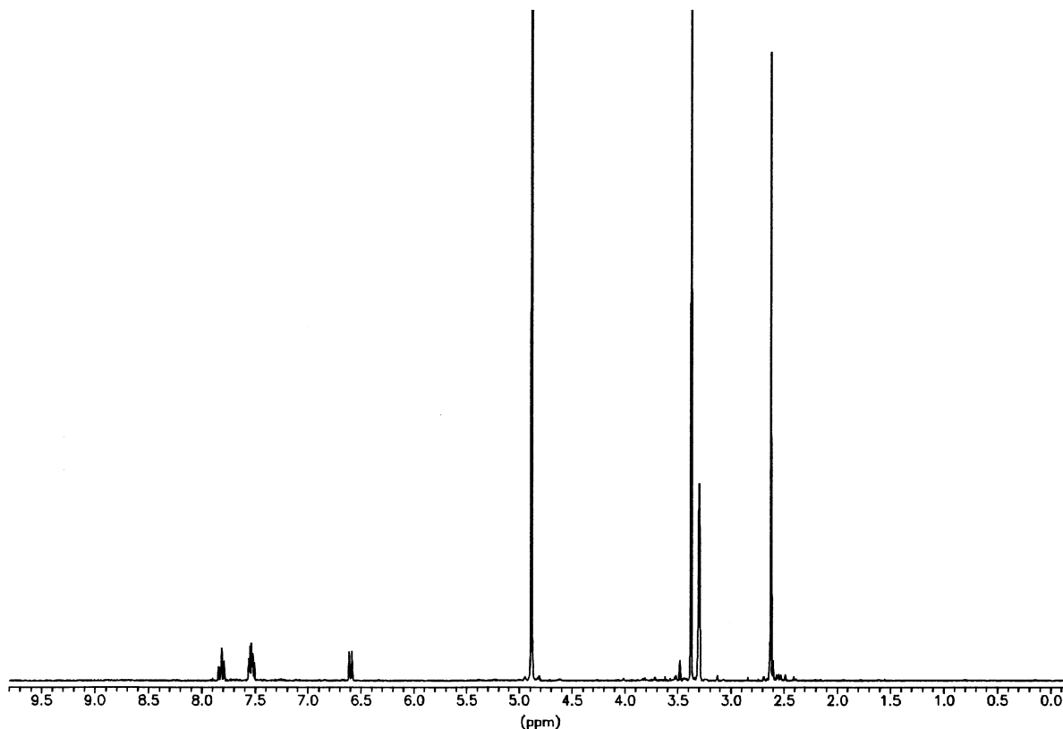
Fig. 31. ^1\text{H} NMR spectrum of nifedipine after photo-oxidation, 300 MHz, solvent methanol- \text{d}_4 .
