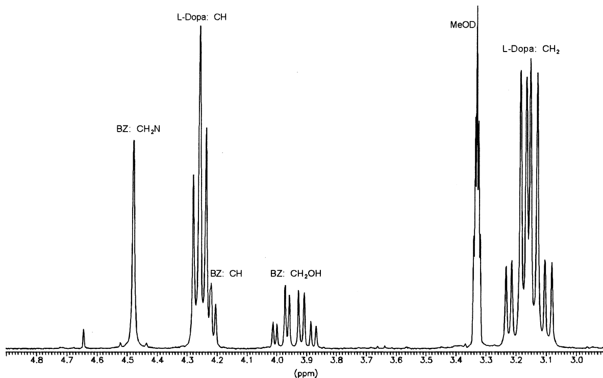
Fig. 34. ^1\text{H} NMR spectrum of Madopar®, \text{CH}_2\text{OH} region, 300 MHz, solvent methanol- \text{d}_4 .
