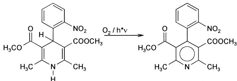
Fig. 29. Nifedipine and its photodecomposition product.
