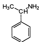
\alpha -methylbenzylamine
