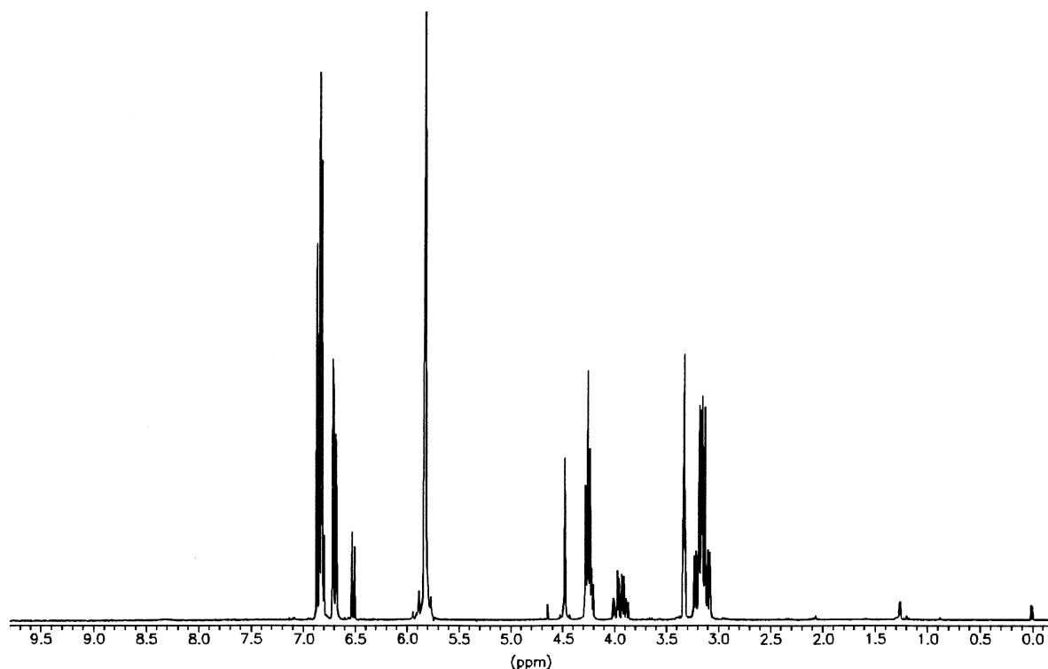
Fig. 33. ^1\text{H} NMR spectrum of Madopar ® , 300 MHz, solvent methanol- \text{d}_4 .
