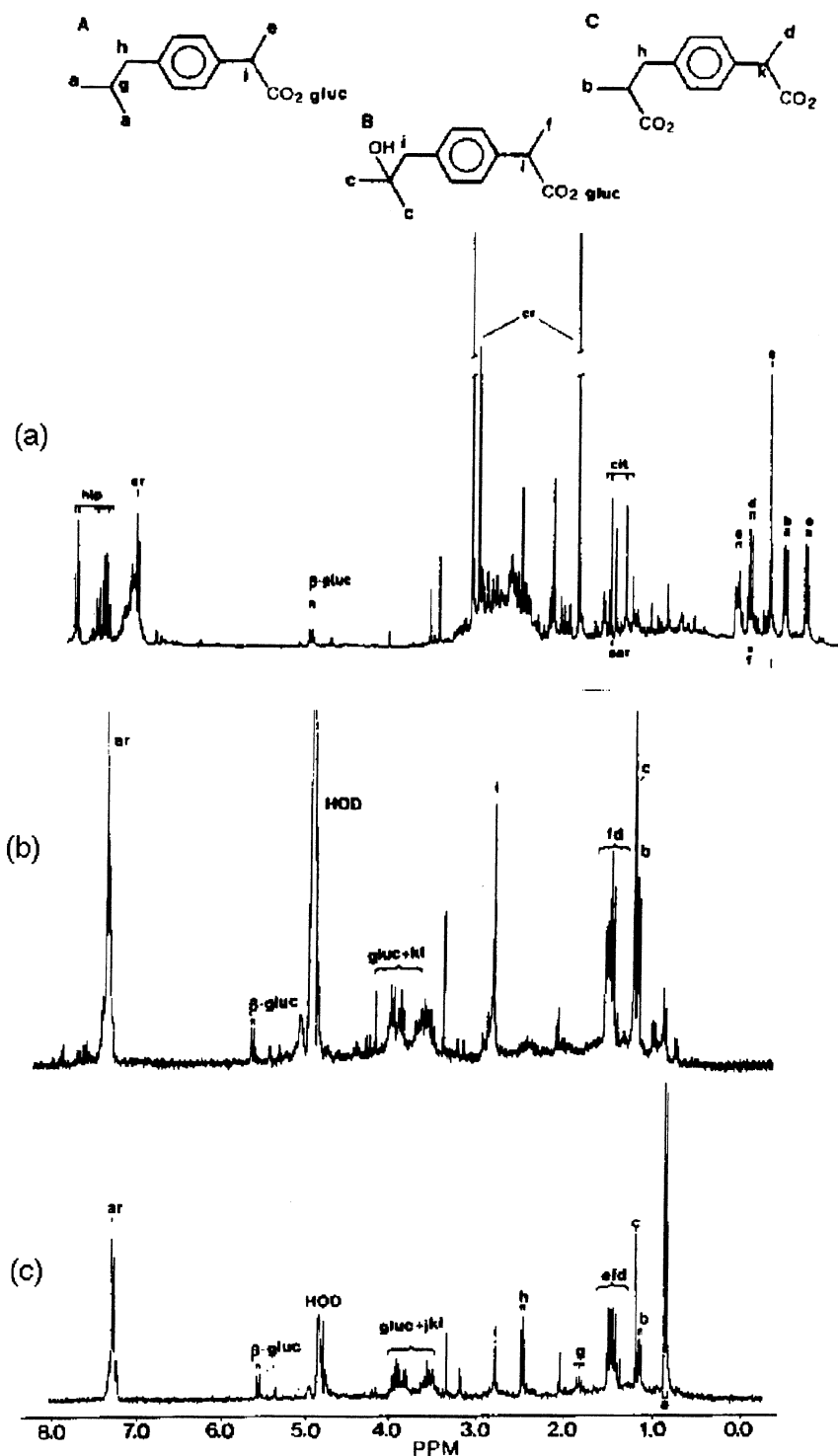
Fig. 43. (a) 250 MHz ^1\text{H} NMR spectrum of a sample of freeze-dried urine (2 ml) obtained from a subject following oral dosing with 400 mg of ibuprofen. The sample was redissolved in \text{D}_2\text{O} for spectroscopy. (b) 200 MHz ^1\text{H} NMR spectra showing the eluates obtained with 40:60 methanol/water (248 scans) and (c) 60:40 methanol/water (66 scans) from a C18 SPE column on which 2 ml of human urine from a sample obtained for the 2–4 h after a 400-mg dose of ibuprofen (Reprinted with permission from Ref. [74], page 2831, Copyright 1997 ACS).
