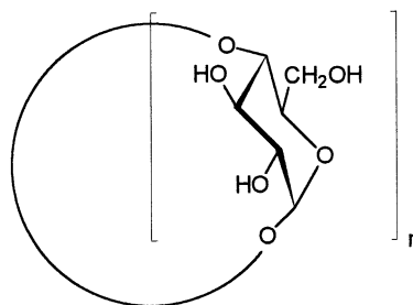
n=6, \alpha -cyclodextrin n=7, \beta -cyclodextrin n=8, \gamma -cyclodextrin
